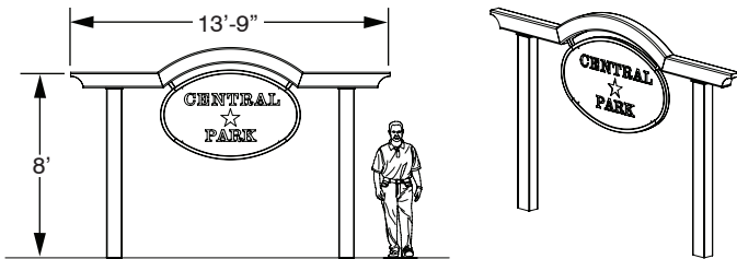
Standard SGB [Double column sign with curved truss]
