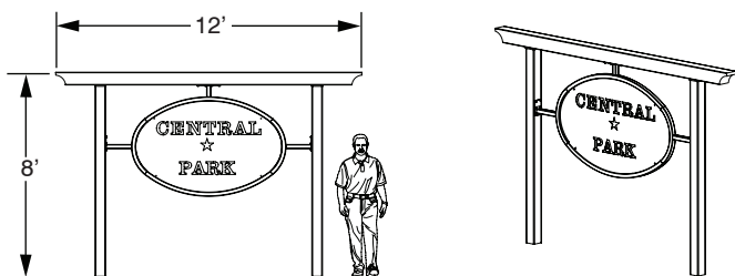
Standard SGC [Double column sign with straight truss]
